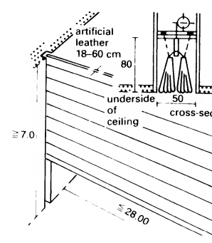
17 Partition curtain
